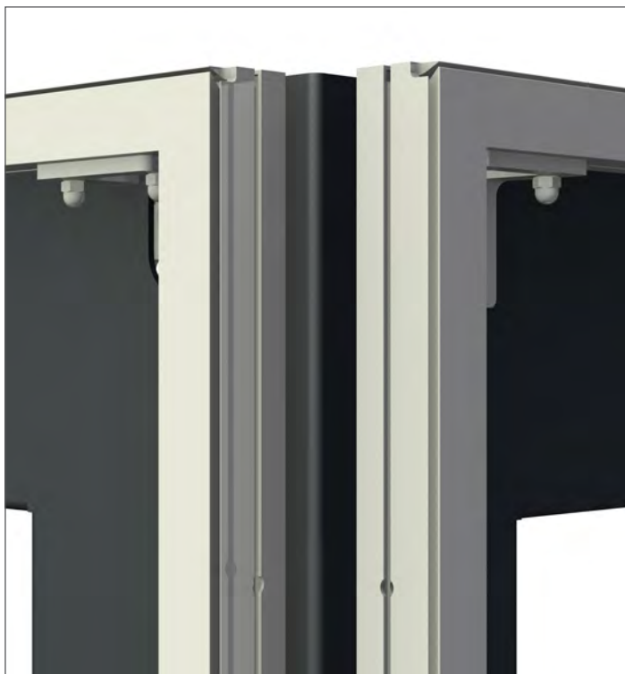
Fixing sets: mounted to the outer container wall.
