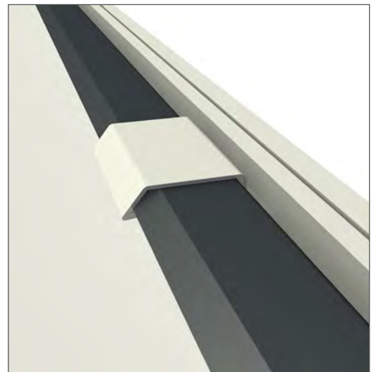
Retaining clips: for maximum stability of the frame
